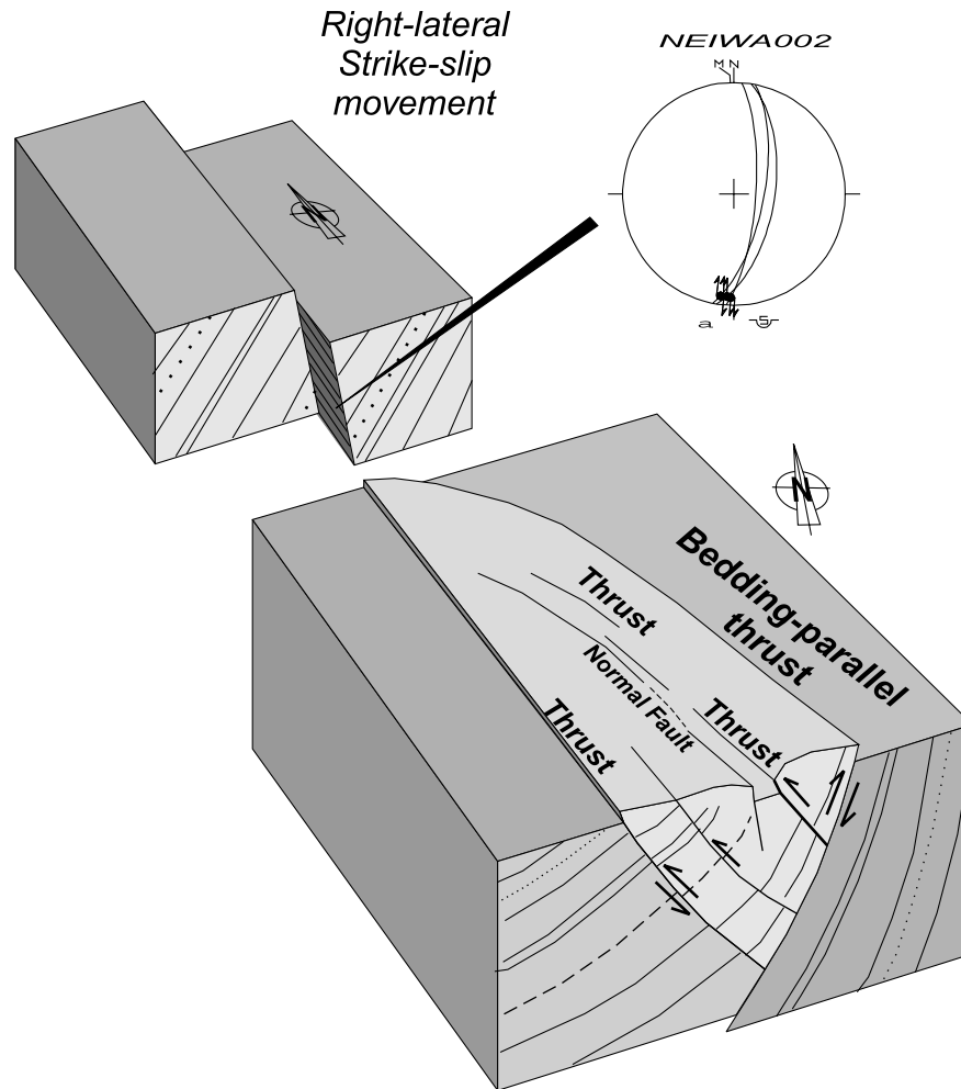
Fig. 12. Simplified block diagrams showing the deformation structure in the eastern part of the Shihkang–Shangchi fault zone. Upper one shows a right-lateral strike-slip movement observed in the outcrop with clear horizontal striations on nearly vertical fault plane. Lower one illustrates a relatively complicated fault system with major bedding-parallel thrust, several antithetic thrusts and normal fault.
